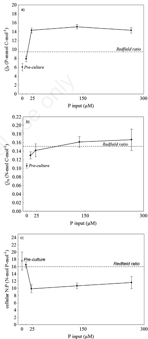
Fig. 1. Behavior of Q_P (a), Q_N (b) and N:P ratio (c) of Cryptomonas pyrenoidifera after 24 h in response to a P gradient in the medium. Value for preculture (open circle) is also shown. Vertical bars represent the propagation of errors of the molar ratios of algae calculated from the standard deviations of the particulate C, N, and P (Bevington, 1969). The Redfield ratio is shown as a broken line for visual reference.
