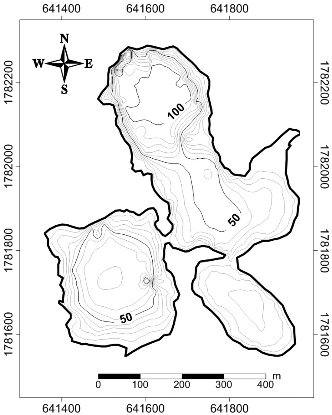
Supplementary Fig. 5. Bathymetric chart of Lake Cinco Lagos, Montebello, Chiapas (UTM).
