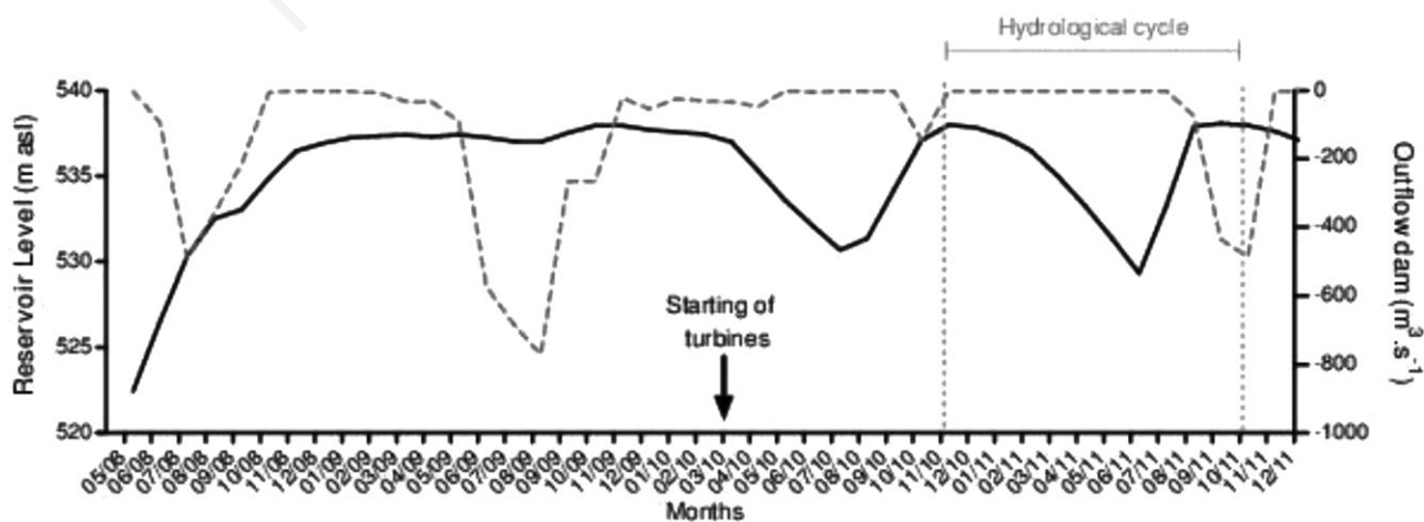
Fig. 2. Graph of hydrological data illustrating the reservoir water level and the outflow from the dam. On the left axis, solid black line corresponds to the reservoir level (m above sea level). On the right axis, dash grey line corresponds to the outflow from the dam site ( \text{m}^3 \text{s}^{-1} ).
