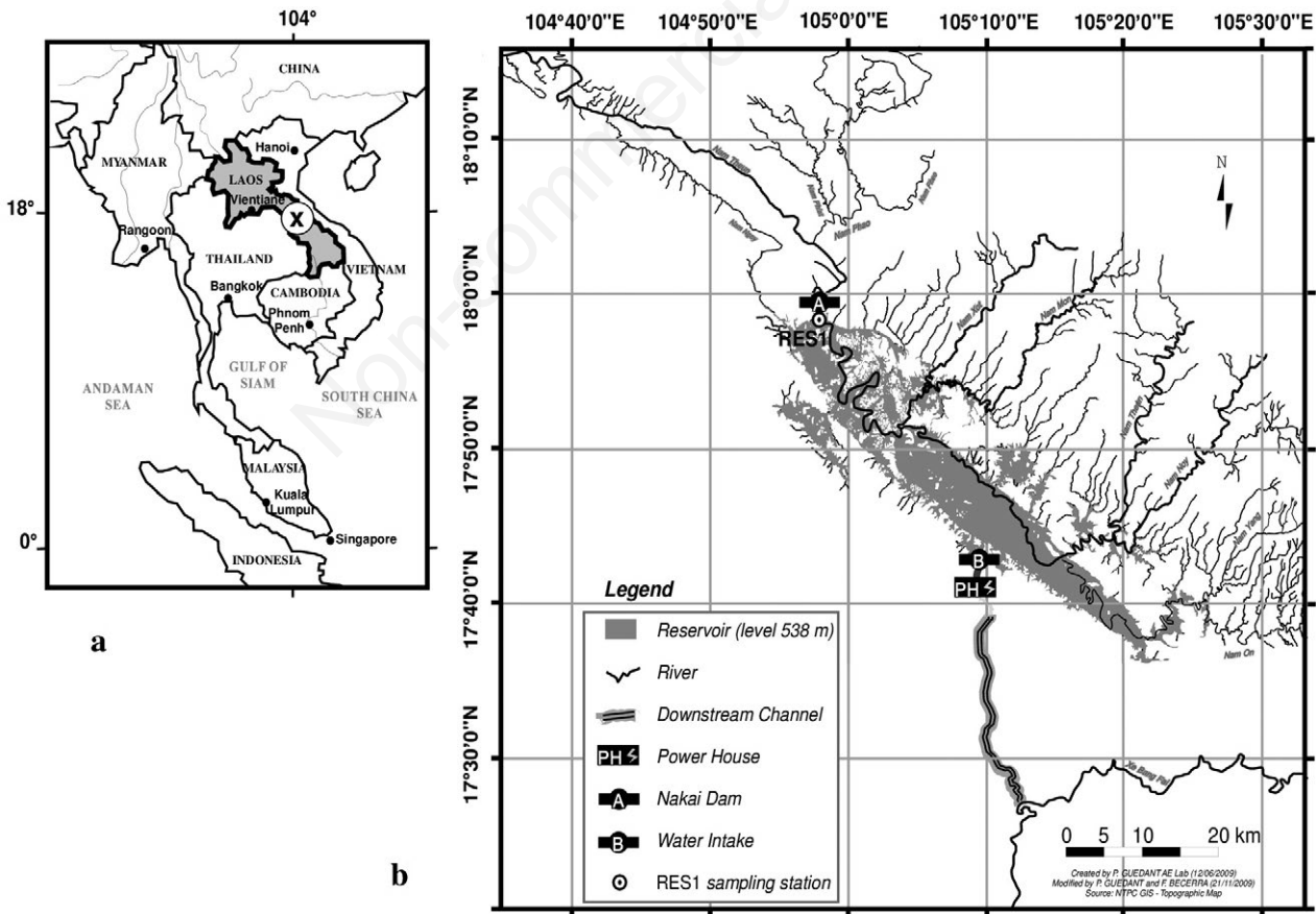
Fig. 1. a) Map of South East Asia with the location of the Nam Theun 2 Reservoir in Laos. b) Map of the NT2 Reservoir and of the sampling site RES1 (Latitude 17°59'51.01"N Longitude 104°57'9.96"E).
