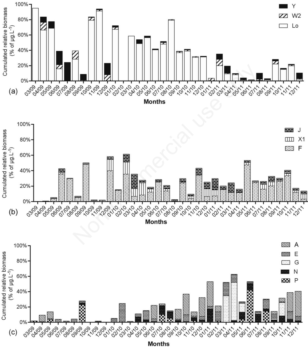
Fig. 5. Evolution of the cumulated relative biomasses expressed in percentage of total biomass (% of \mu\text{g L}^{-1} ) for the different assemblages identified overt the study. a) Relative biomasses of some pioneers functional groups (Y, Lo and W2). b) Relative biomasses of some transitional functional groups (F, X1 and J). c) Relative biomasses of some functional groups (A E G N and P).
