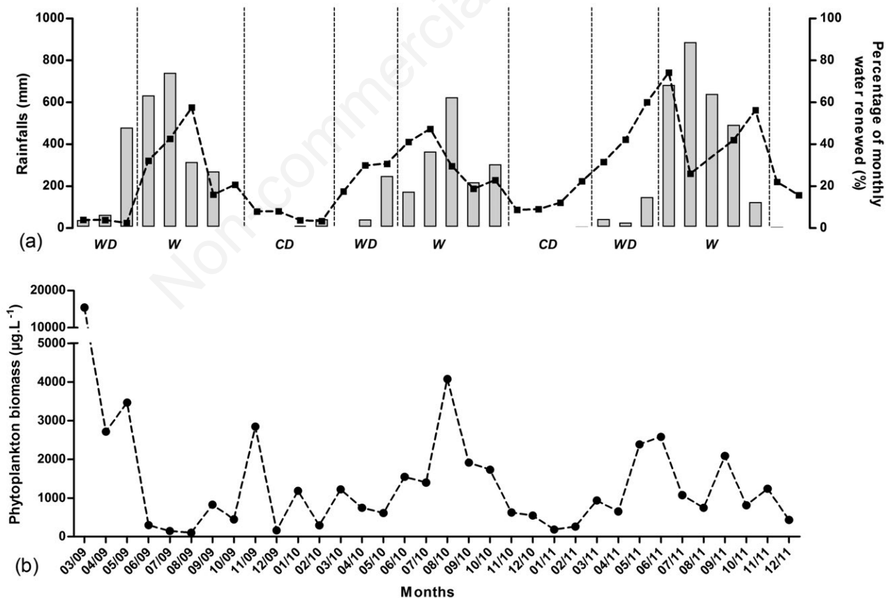
Fig. 3. a) Hydrological characteristics of the NT2 Reservoir following the percentage of monthly water renewed (black square) with rainfall (grey bar) and b) phytoplankton biomass evolution (black dot) from March 2009 to December 2011. CD, cool dry season; WD, warm dry season; W, wet season.
