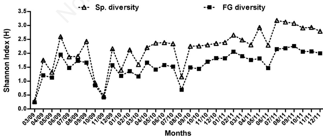
Fig. 4. Dynamic of the Shannon-Weaver diversity index (black dot) for species (black triangle) and functional groups (black square) from March 2009 to December 2011.
