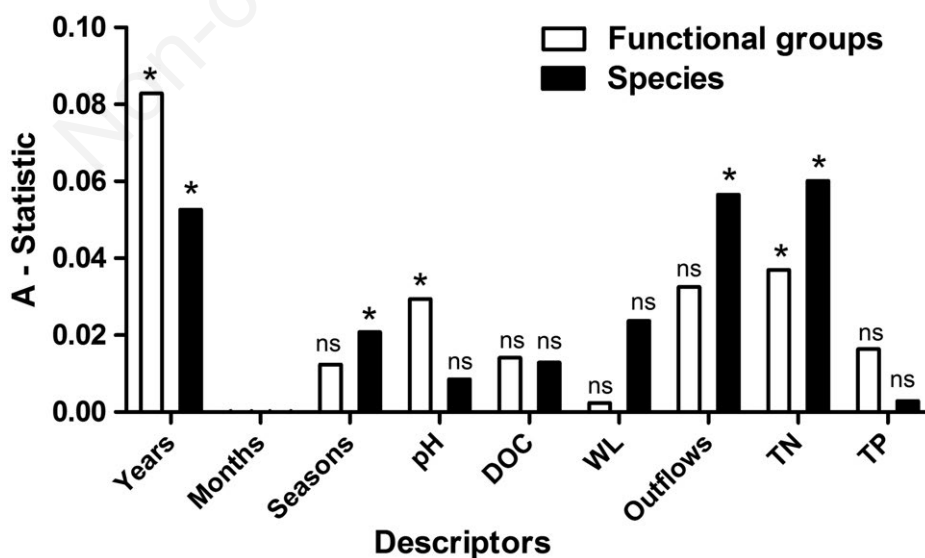
Fig. 6. Temporal and environmental parameters structuring the phytoplankton communities when expressed as species biomass or functional-groups biomasses. The A-statistic (calculated by an MRPP) provides an assessment of the communities heterogeneity for temporal descriptors as years, months, seasons, for chemical parameters as pH, total nitrogen (TN), total phosphorous (TP), dissolved organic carbon (DOC), and hydrological parameters as water level (WL), outflows from the dam (Outflows).
