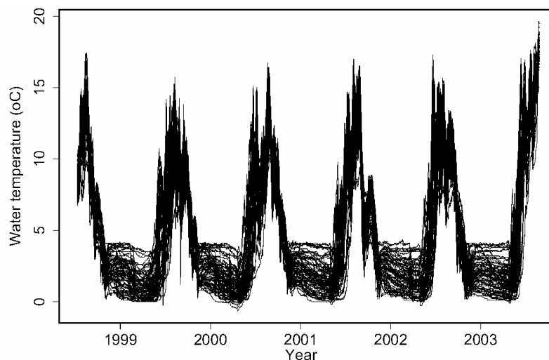
Fig. 2. Suite of thermistor logs in the epilimnion layer of the NT lakes. Daily mean temperatures are plotted for 86 thermistors.
