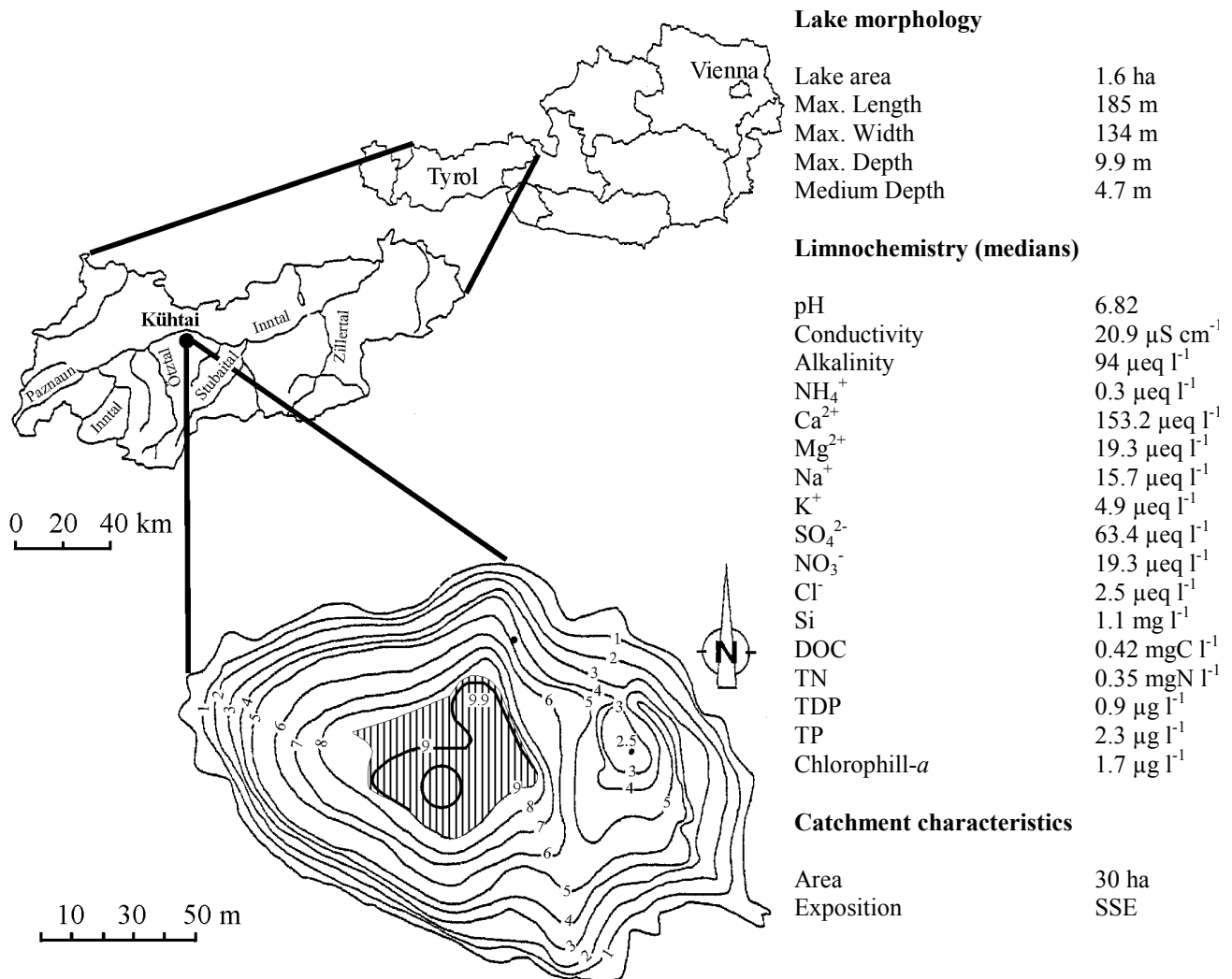
Fig. 1. Geographical position, bathymetric map and characteristics of Gossenköllesee. The shaded area indicates soft sediment. The circle illustrates the coring position of all cores presented in this paper.
