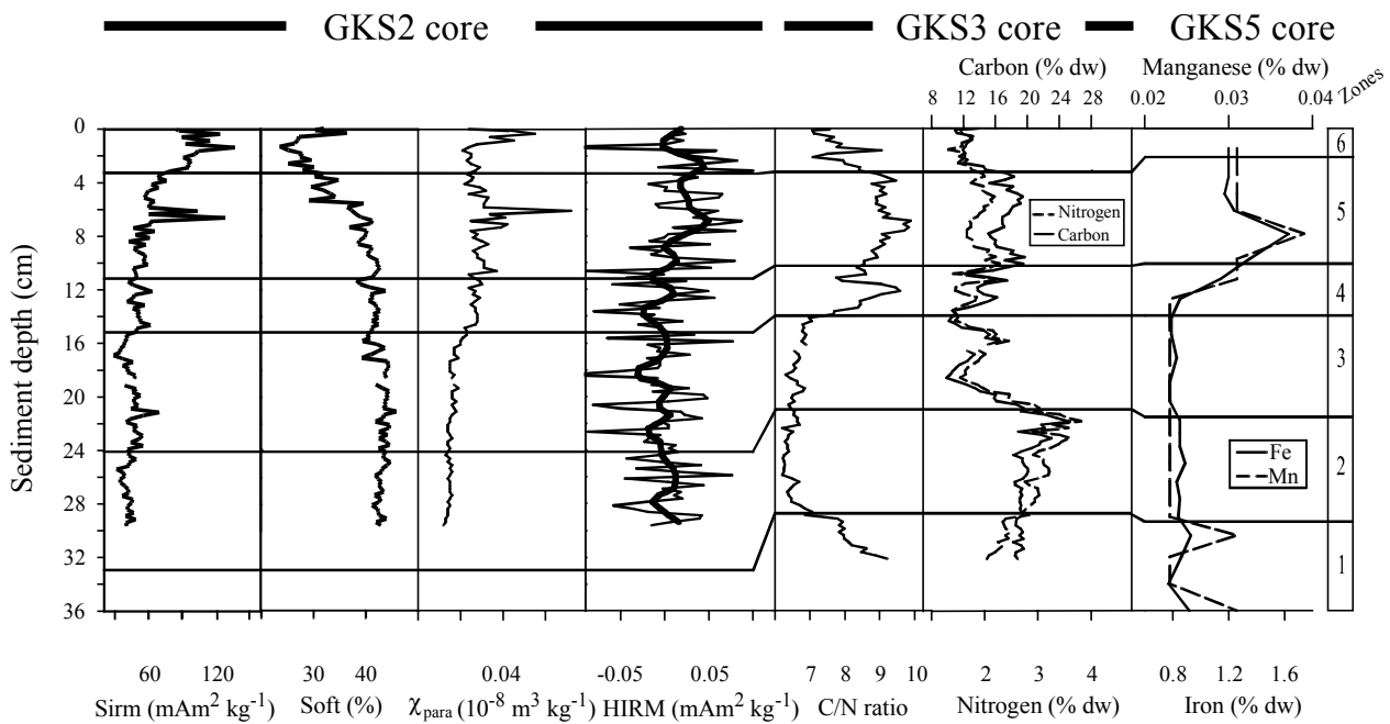
Fig. 3. Profiles of SIRM, SOFT%, \chi_{\text{para}} , HIRM, carbon, nitrogen, C/N ratio, iron and manganese. Zone boundaries were set according to a combined interpretation of all results.
