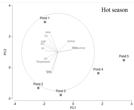
Fig. S1. Principal Component Analysis (PCA) of environmental variables among five ponds in each season.
