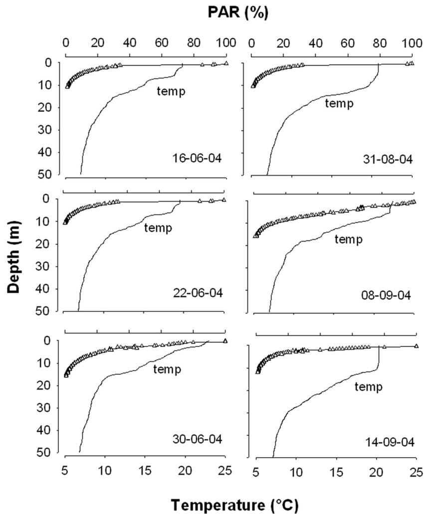
Fig. 1. Profiles of temperature (line) and percentage of surface PAR (triangles) in the two study periods, in Lake Maggiore 2004.
