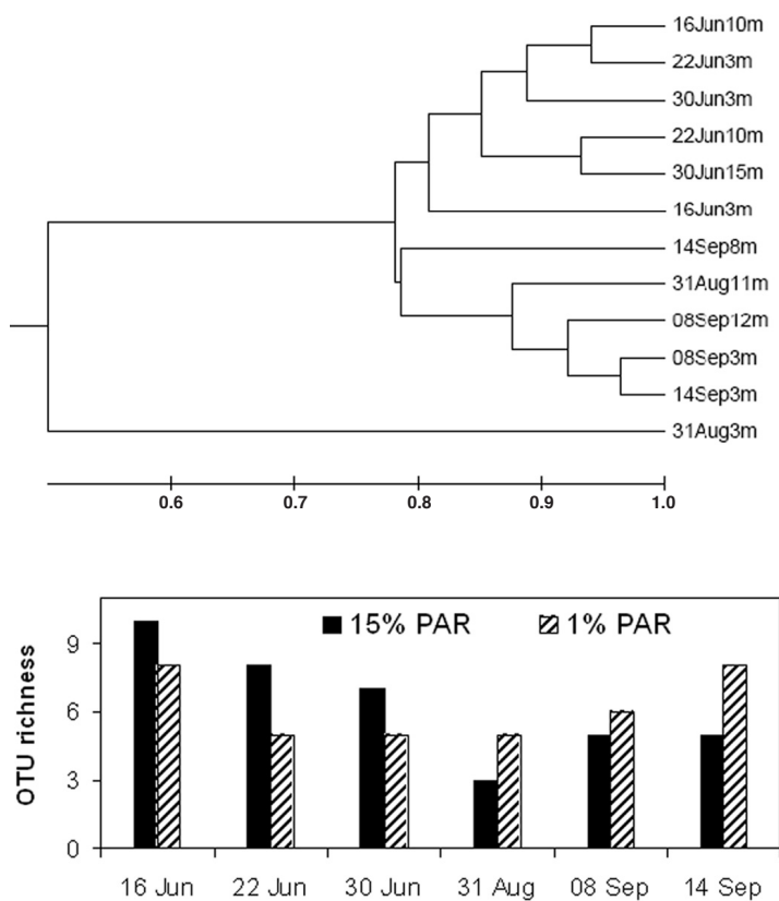
Fig. 4. Cluster analysis of picocyanobacteria communities based upon significant (> 0.5 % of total lane brightness) DGGE bands. Similarities are expressed as the Bray-Curtis Coefficient, which compares the relative contribution of single OTUs to the total amplified DNA of each band, when making pairwise comparisons between samples. Clustering was performed with UPGMA. Richness in bands of each sample is reported by grouping 15 % PAR (3 m) samples and 1 % PAR (between 8 and 15 m depth).
