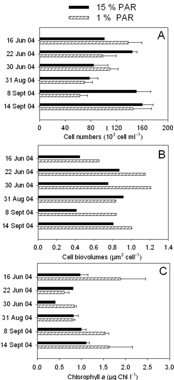
Fig. 2. Numbers of picocyanobacteria ( 10^3 \text{ cells ml}^{-1} ) (A), cell volume ( \mu\text{m}^3 \text{ cell}^{-1} ) (B), Chlorophyll a concentrations ( \mu\text{g l}^{-1} ) (C), at the two depths during the two study periods, in Lake Maggiore 2004.
