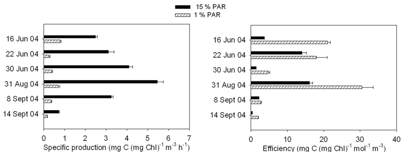
Fig. 3. Chlorophyll specific production ( \text{mg C (mg Chl)}^{-1} \text{ m}^{-3} \text{ h}^{-1} , left) and photosynthetic efficiency ( \text{mg C (mg Chl)}^{-1} \text{ mol}^{-1} \text{ m}^{-3} , right), measured in the pico fraction at the two depths on six dates, in Lake Maggiore 2004.
